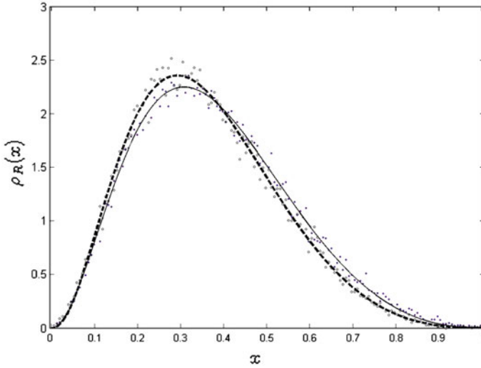
Fig. 4. Fit of the invariant density for the evolution under T (solid line) and under T_\epsilon , \epsilon = 0.5 , (dashed line)
