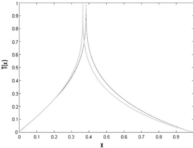
Fig. 3. T_{\epsilon} (thick line), T (thin line)
