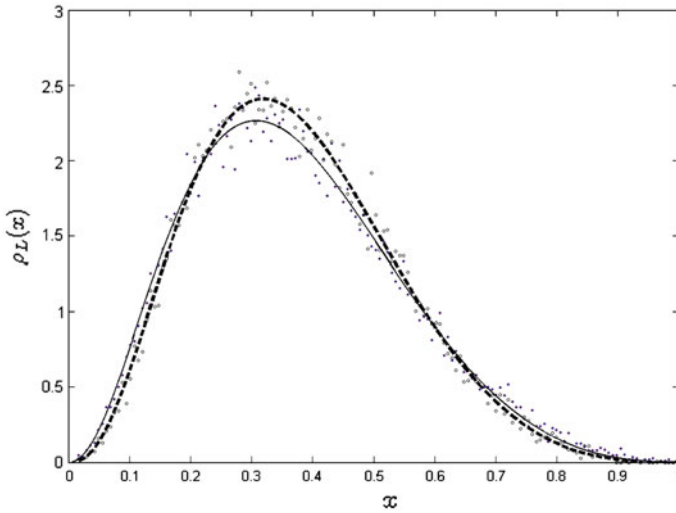
Fig. 7. Fit of the invariant densities for the evolution under T (solid line) and under T_\epsilon^- (dashed line)
