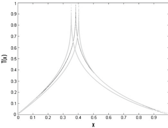
Fig. 5. T (thin line), T_\epsilon^+ (thick line to the left of T ), T_\epsilon^- (thick line to the right of T )
