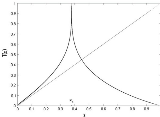
Fig. 1. Normalized Lorenz cusp map for the Casimir maxima
