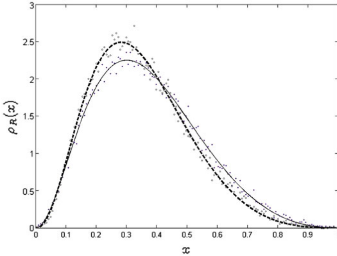
Fig. 6. Fit of the invariant densities for the evolution under T (solid line) and under T_\epsilon^+ (dashed line)
