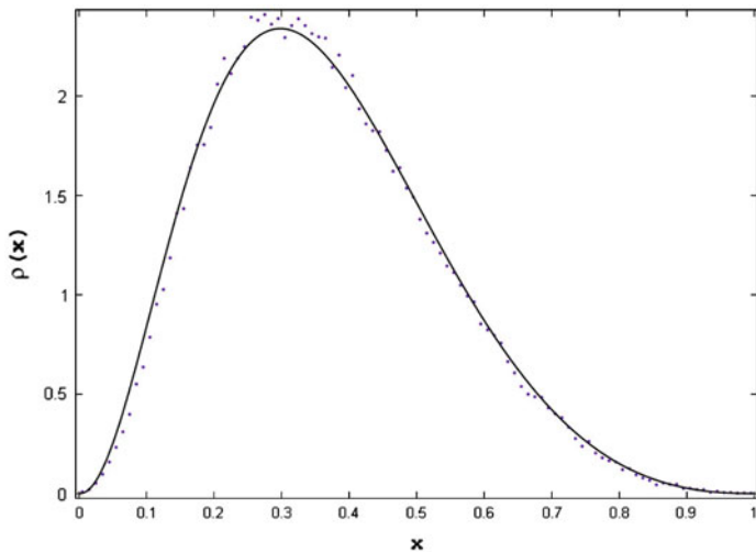
Fig. 2. Fit of the invariant density \rho(x) for the map T with the function given in (83)
